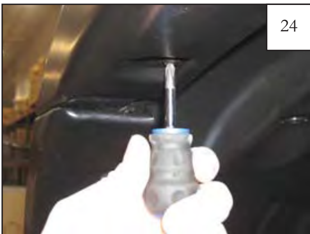
Install a supplied Screw (SW1-0050) through hole in flare and into Clip installed in step 22. 4 places.
